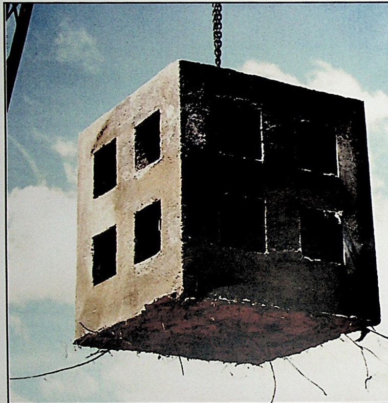
Figure 5 : A side view of a 3.2 tonnes concrete anchor
