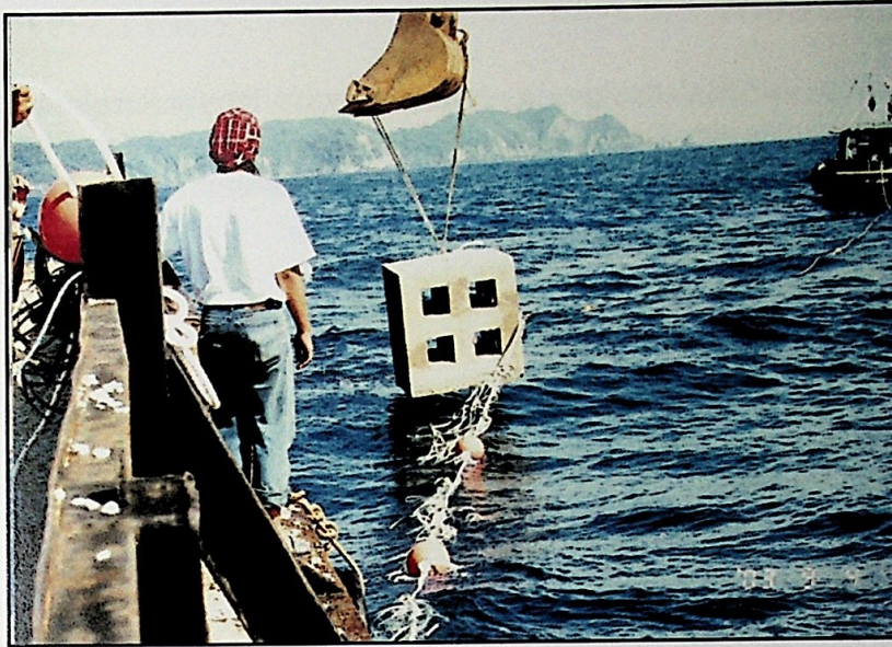
Figure 17 : Another style of the anchor-last method applied during the deployment of ARFADs
