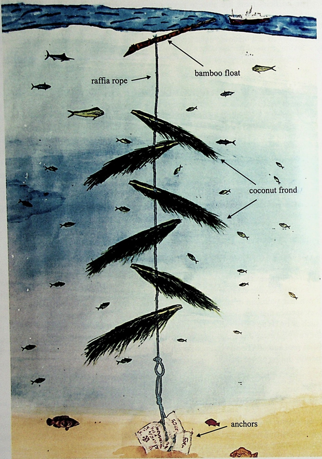
Figure 1 : An unjam, a kind of FADs commonly used by Malaysian fishermen
