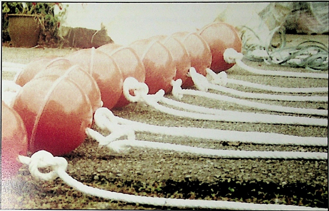
Figure 3 : The submerged floats used for these ARFADS. The size of each float is 30.4 cm diameter with a 2.5 cm hole in the middle.
