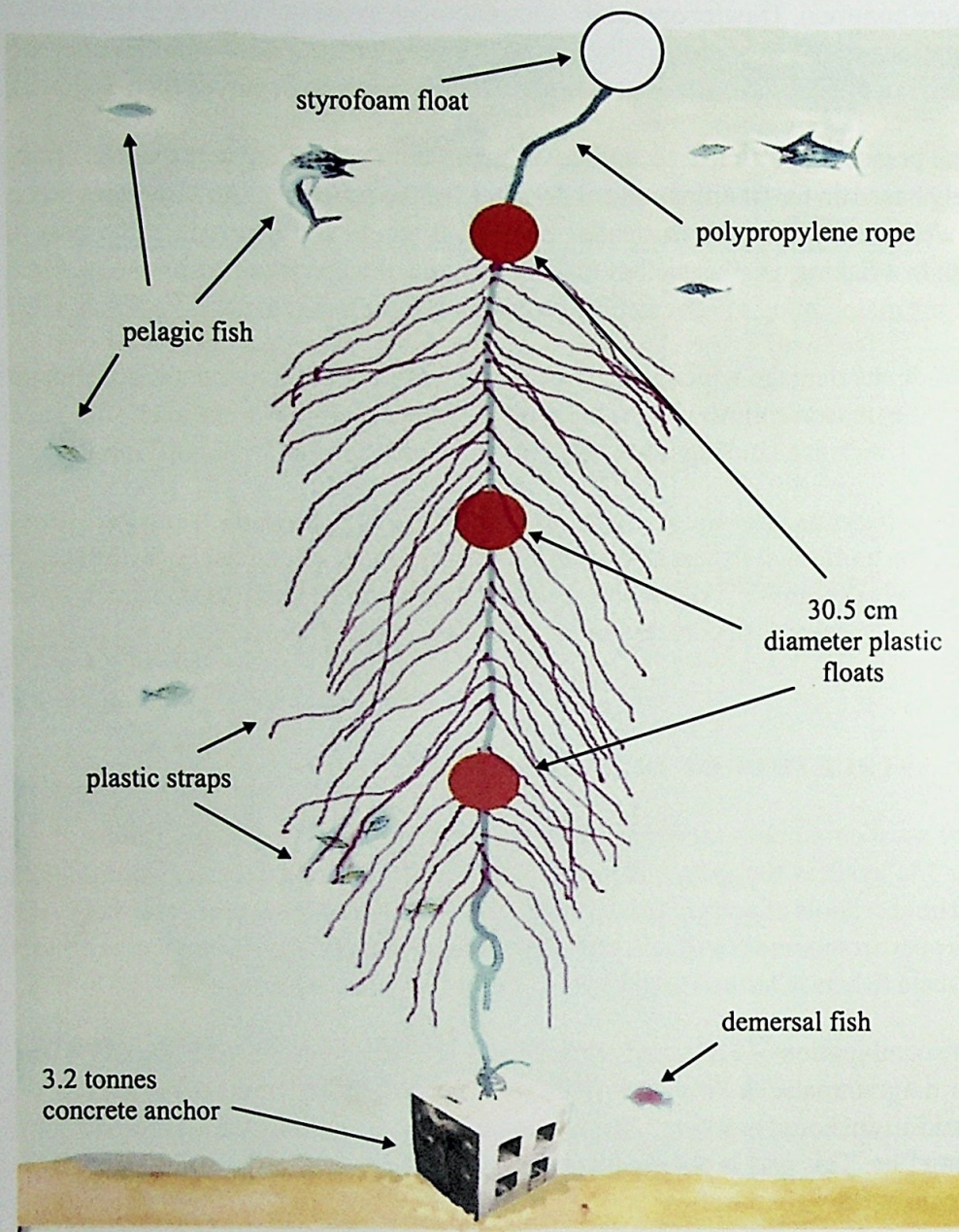
Figure 2 : A durable ARFADs that is recommended for attracting both pelagic and demersal fish species in coastal areas
